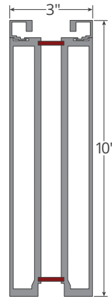
10" Bottom Rail**
